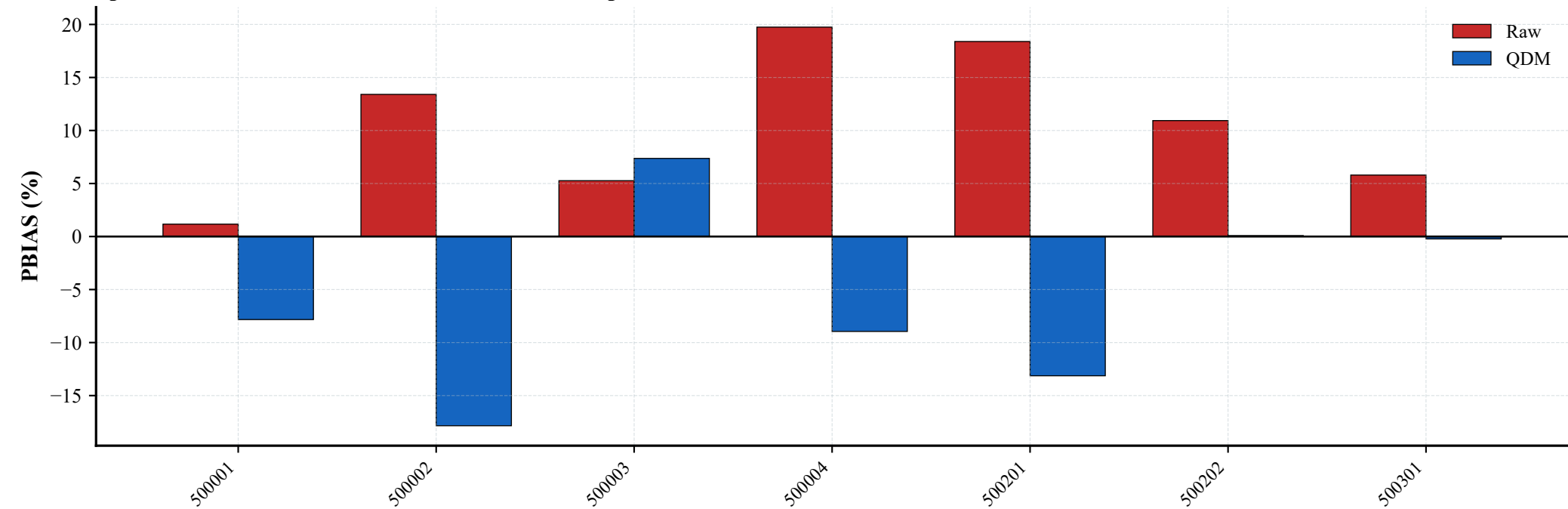
Spatial variation of PBIAS across stations — independent validation
